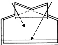
(b) butterfly rooflight with translucent ceiling
